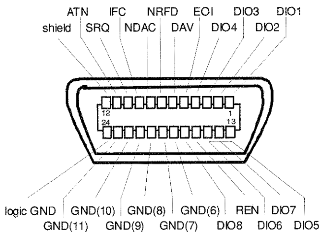
Fig. A-1 Contact Assignment of the IEC-bus socket
