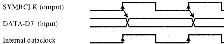
Fig. 2-51 External parallel data and symbol clock. SYMBOL CLOCK = High marks the LSB. A status change of DATA and SYMBOL CLOCK should be performed synchronously.
