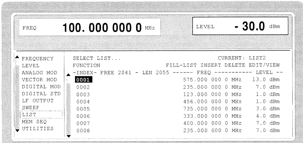
Fig. 2-131 Menu List - EDIT page
