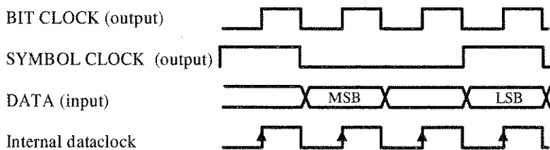
Fig. 2-49 External serial data, internal clock signals
